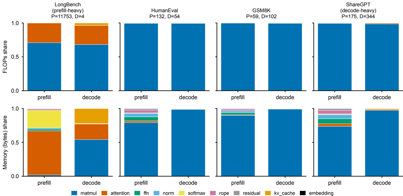
Op-category composition — Llama-3.1-8B (matmul dominates compute & memory; attention rises in long-context prefill)
