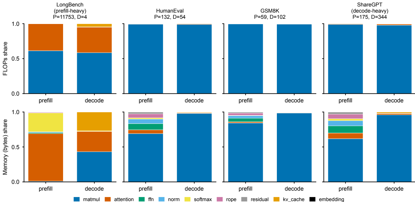
Op-category composition — Llama-3.2-1B (matmul dominates compute & memory; attention rises in long-context prefill)
