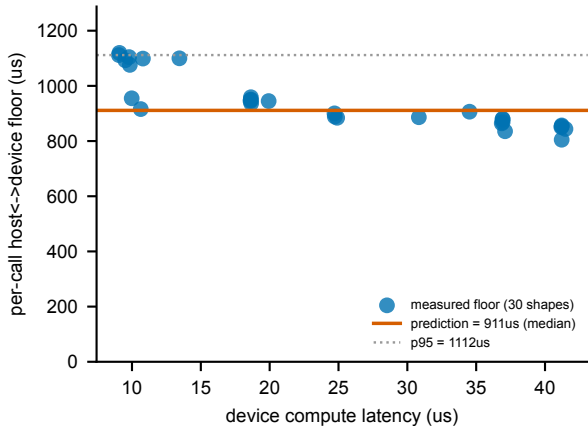
M2 PCIe floor: measured vs fixed 911us
