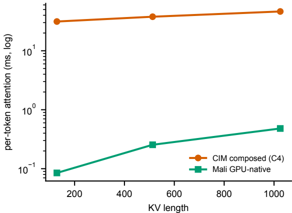
P7 CIM penalty vs GPU offload (~2 orders, 96-370x)
