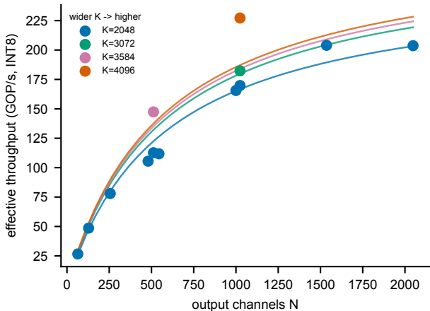
P2 CIM G_{\text{eff}}(N,K) : meas (dots) vs 2D fit (lines)
