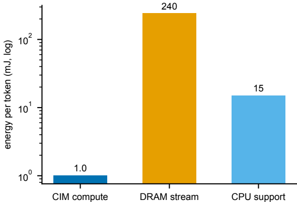
M7 8B decode energy (memory-dominated; 0 flips \pm 20\% )
