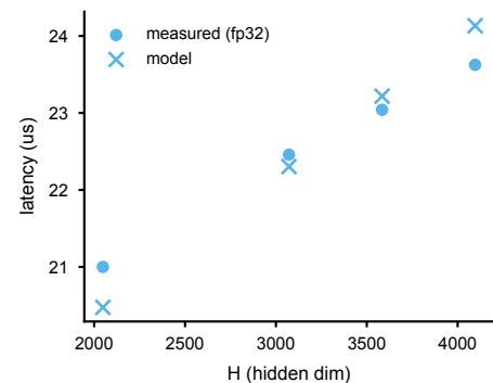
rmsnorm
