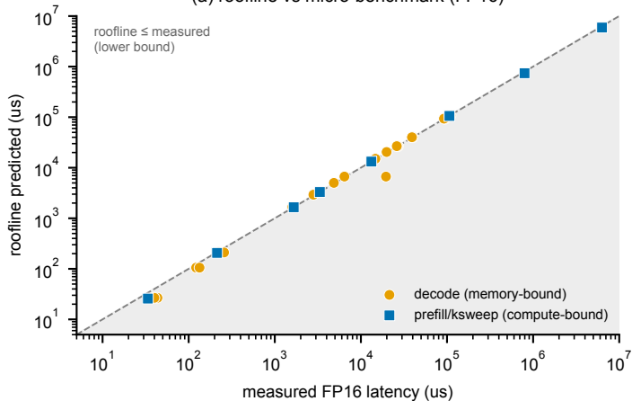
(a) roofline vs micro-benchmark (FP16)
