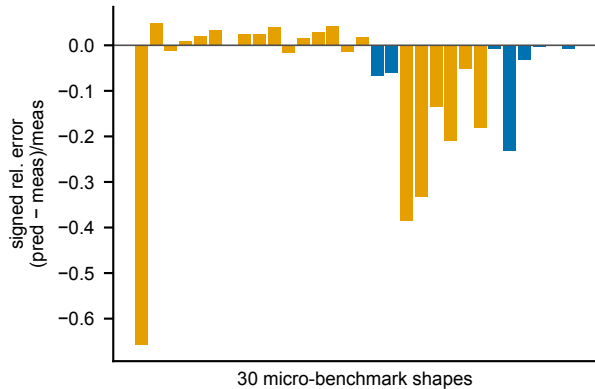
(b) median|err|=3%, p95=36%
