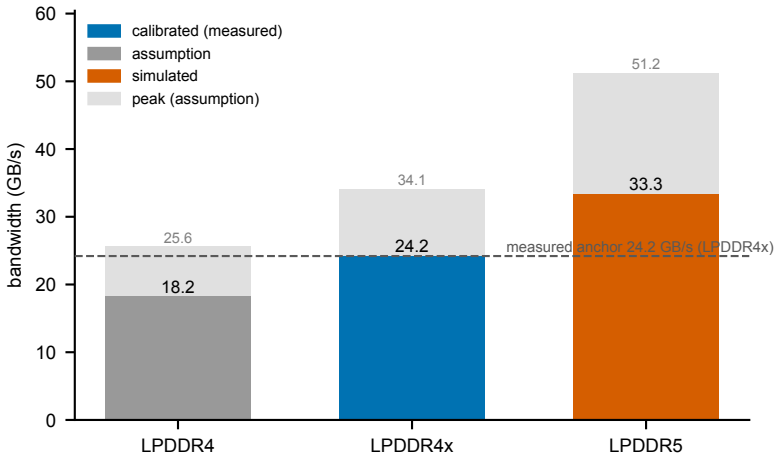
M2 host-DRAM effective bandwidth — 3 swappable specs (LPDDR4x = measured 24.2 anchor; LPDDR5 = sim 0.65 discount)
