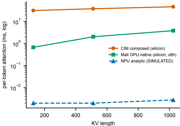
N2 attention offload — CIM/Mali silicon (solid) vs NPU (dashed, sim)
