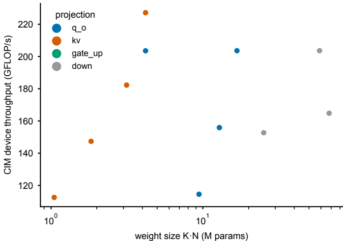
CIM matmul throughput vs op (decode M=1) tiled ops amortise differently
