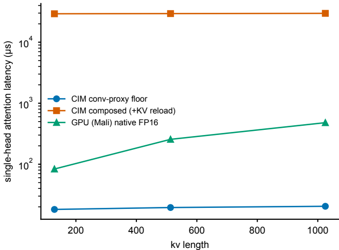
Attention: CIM penalty vs GPU native (motivates offload)
