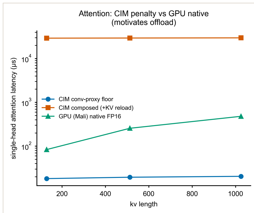
Figure 4. Single-head attention latency vs kv length: CIM conv-proxy floor (compute only, misleadingly fast), CIM composed (+KV reload, the real ~29 ms penalty), and GPU-native FP16 (Mali, 80-500 μs). The two-order-of-magnitude gap motivates assigning attention to GPU/NPU.
