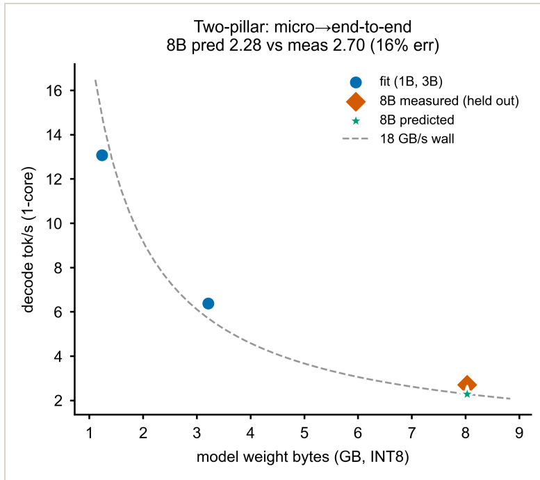
Figure 5. Two-pillar hold-out. Effective decode bandwidth fit on 1B and 3B predicts the held-out 8B decode tok/s within 16 % of the measurement . The residual is real size-dependence (smaller models stream weights less efficiently), not a fit artifact.
