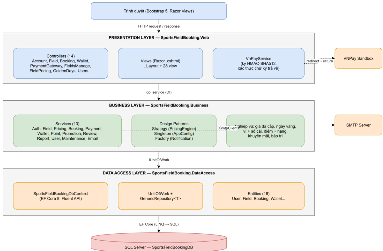
Hình 1.1 - Software Architecture (3-layer)
