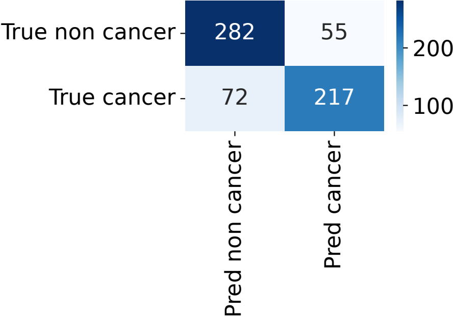
Confusion matrix at Youden optimal t
