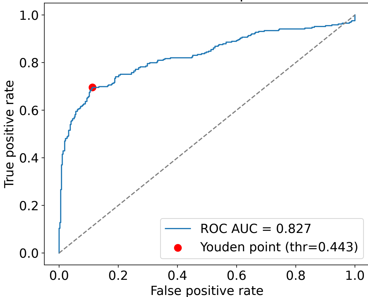
ROC curve with Youden optimal threshold
