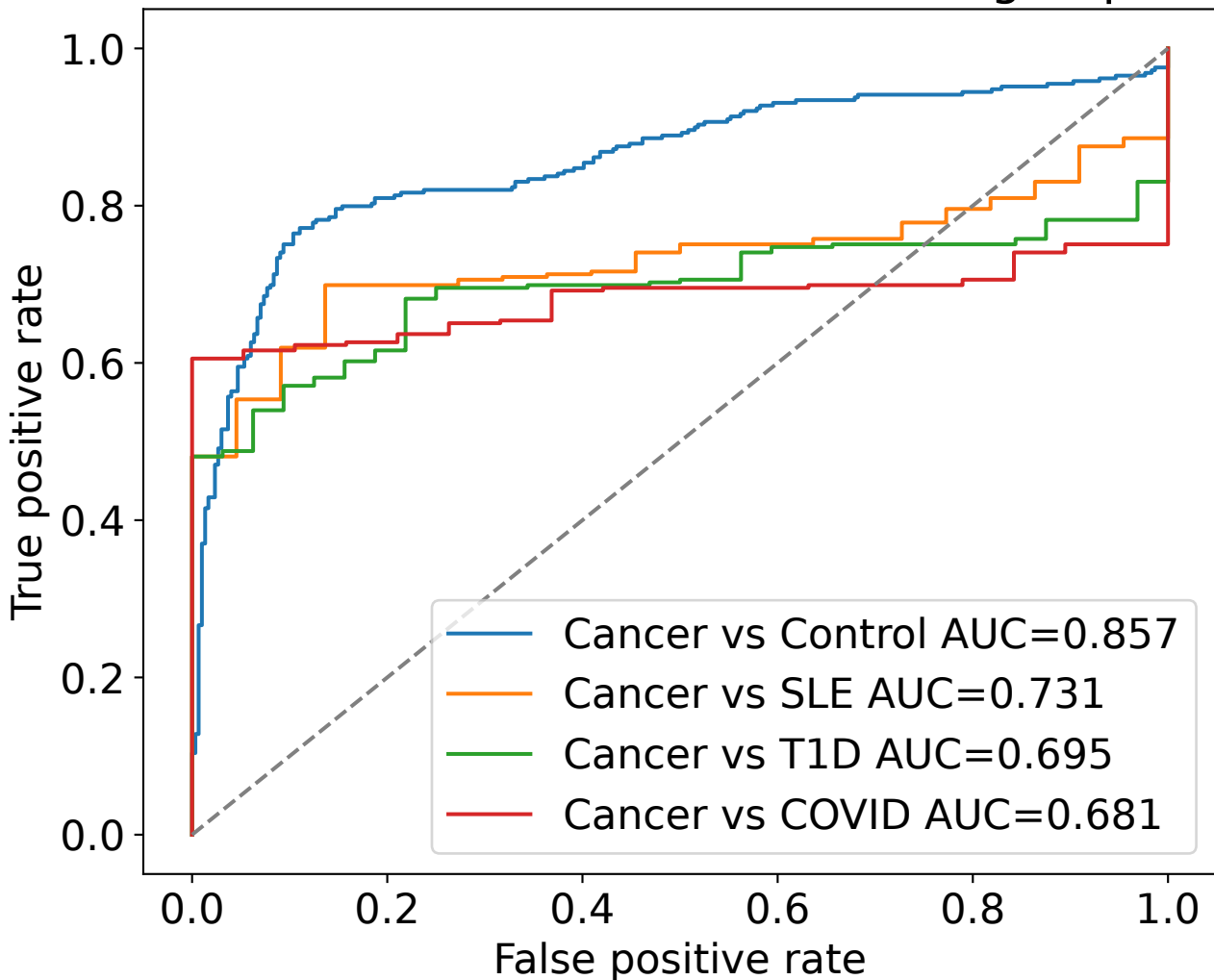
ROC curves for Cancer vs other groups
