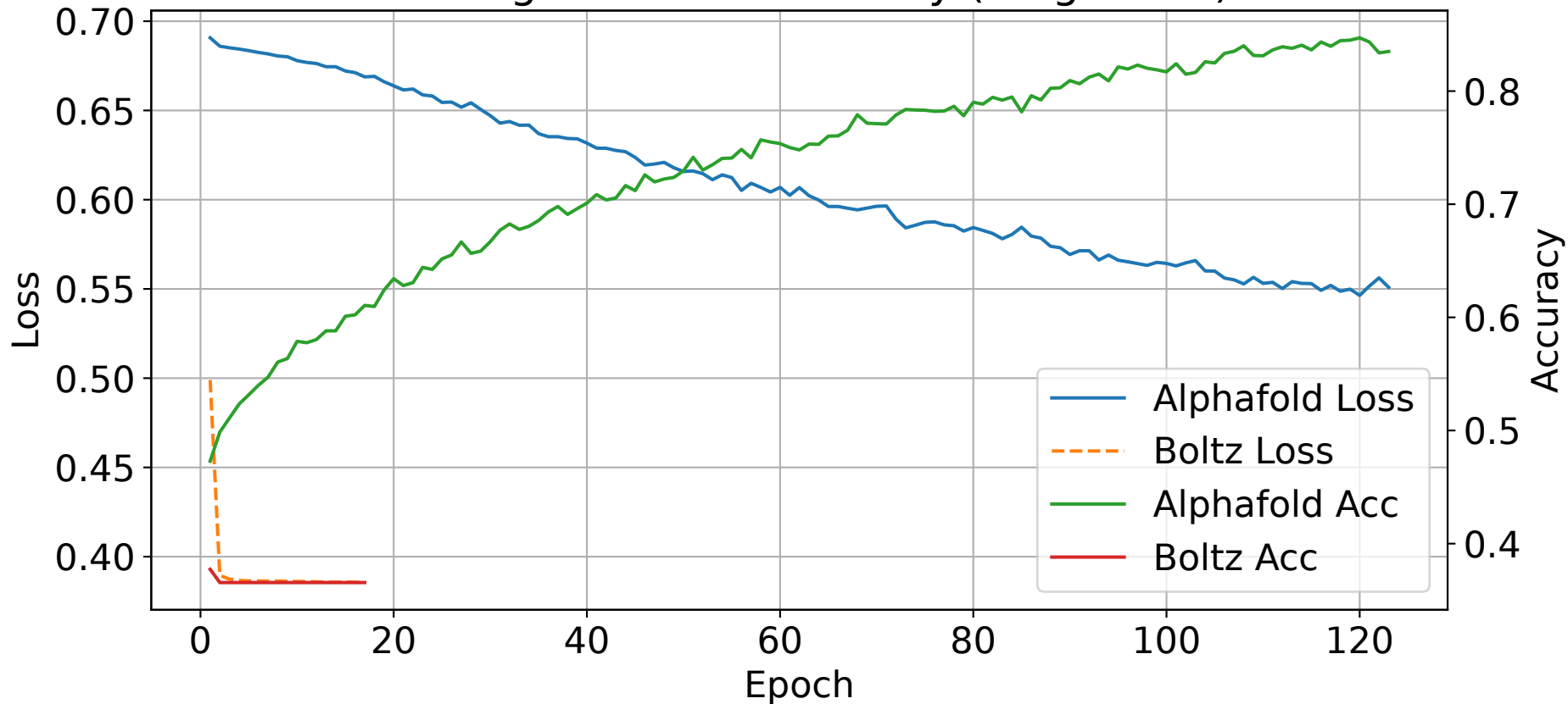
Training Loss and Accuracy (Single Plot)
