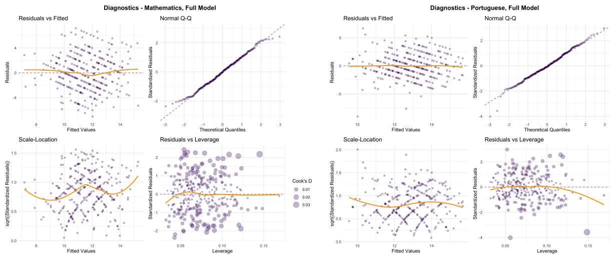
(a) Mathematics — Full Model
