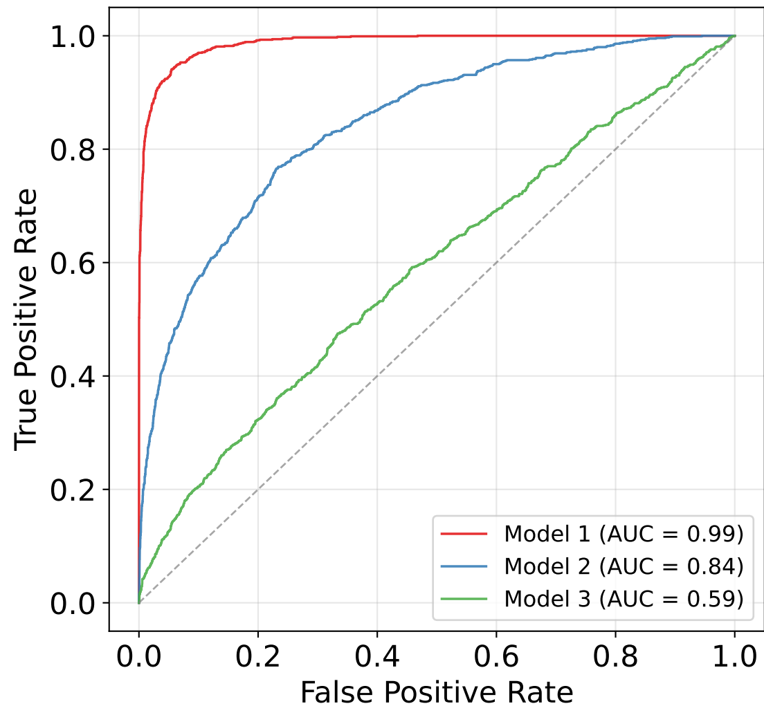
ROC Curve
