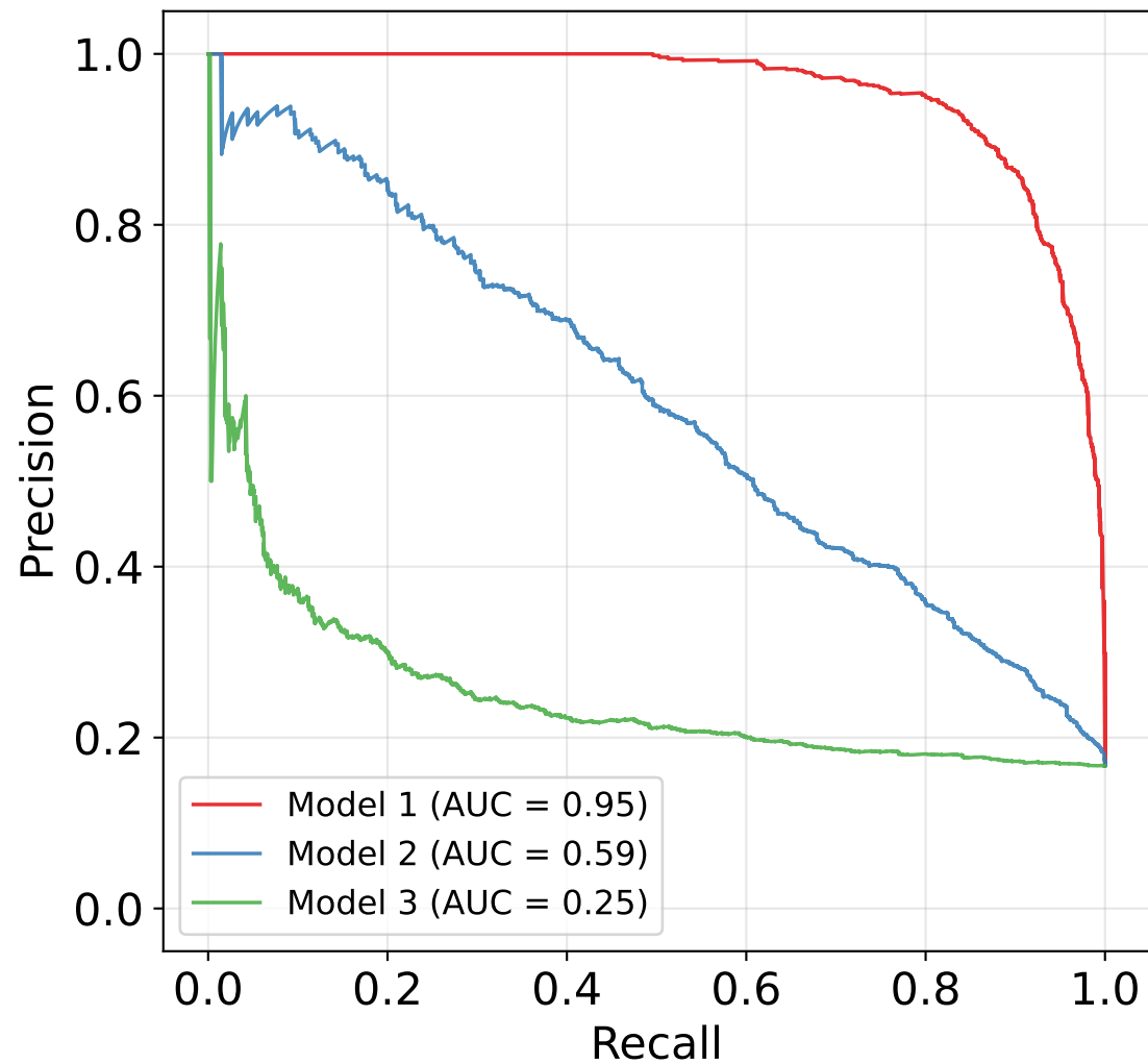
Precision-Recall Curve
