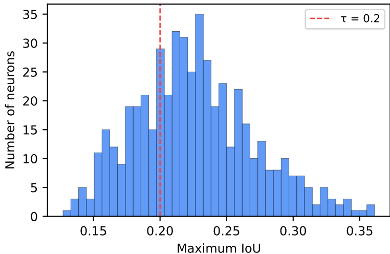
Neuron Specialisation (layer4.1.conv2)
