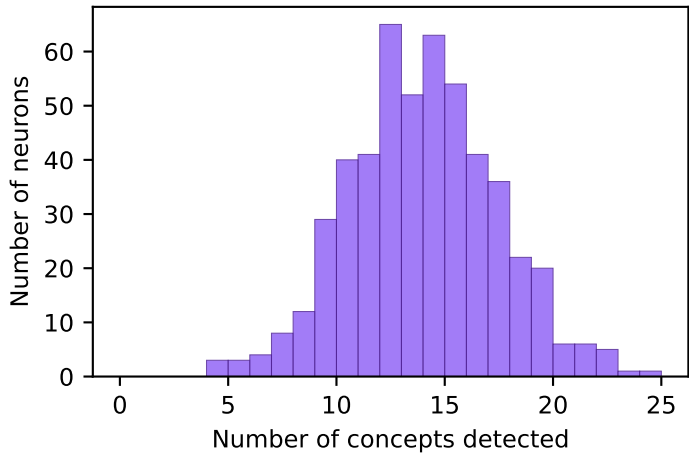
Polysemanticity Distribution
