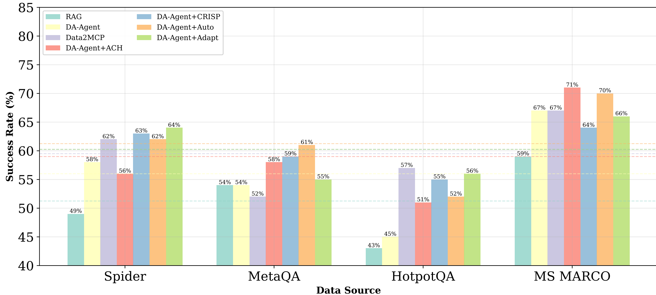
Multi-Source Retrieval: Detailed Performance Comparison
