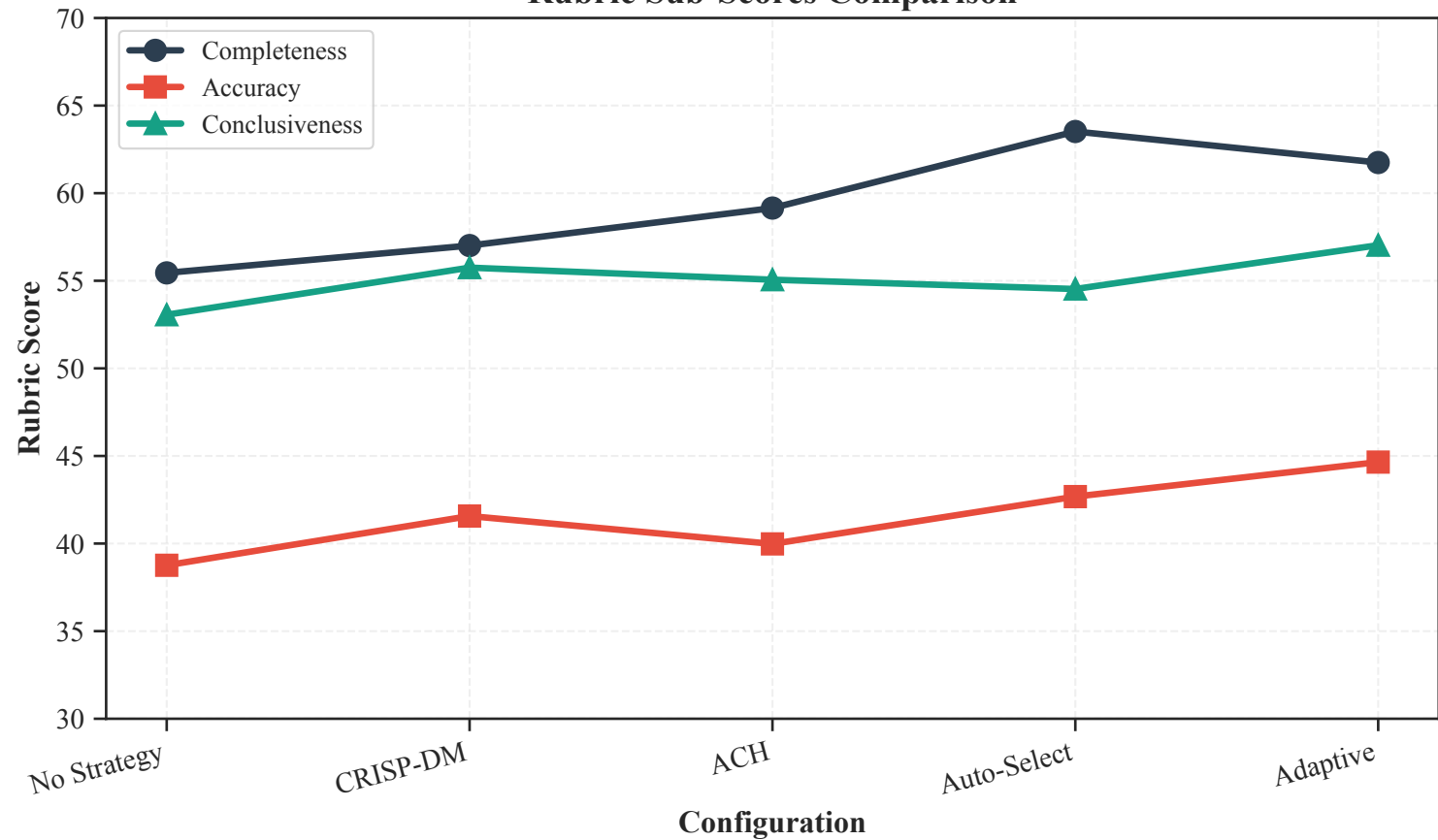
Rubric Sub-Scores Comparison
