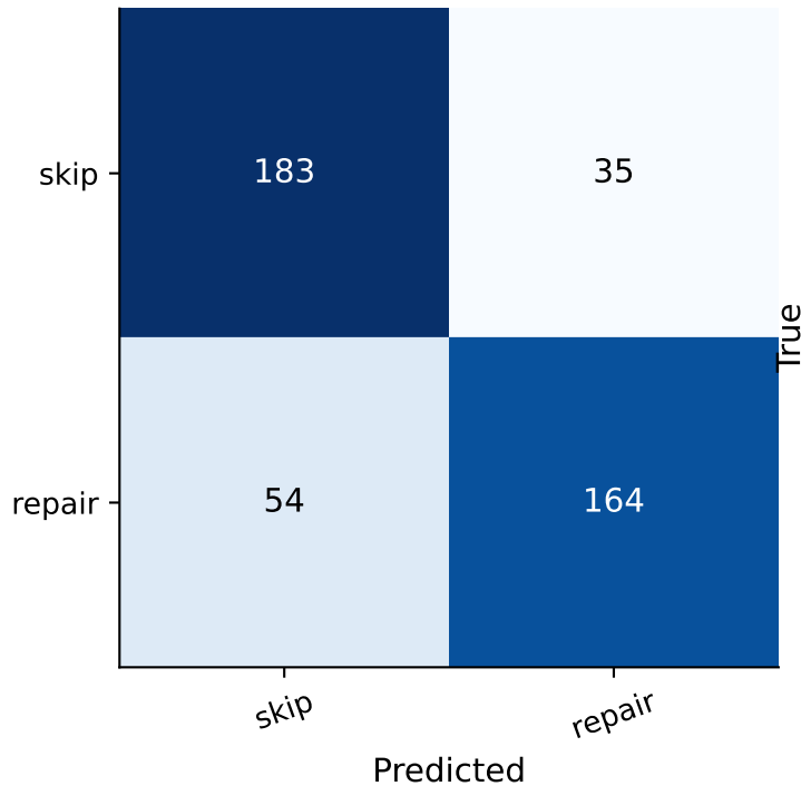
Repair trigger p_{repair}
