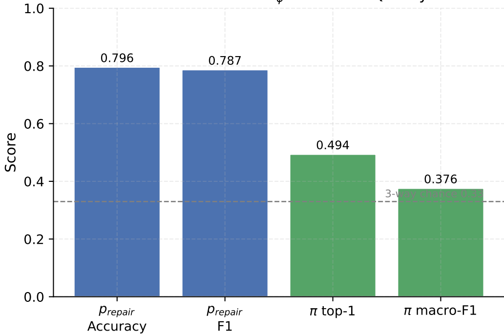
Decision Network f_\phi Prediction Quality
