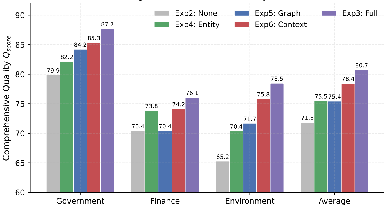
Single-Scale Ablation vs Full System
