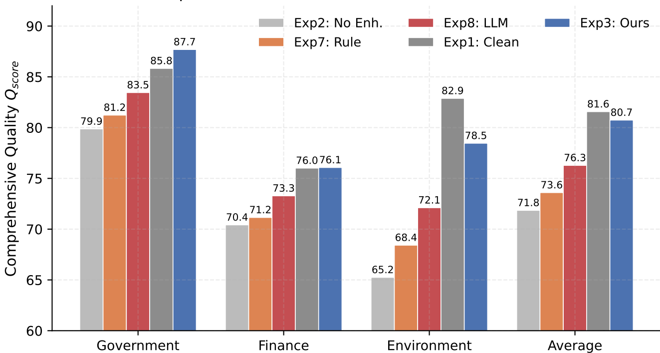
Comprehensive Results Across Methods and Domains
