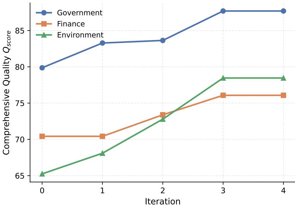
Per-Iteration Convergence (plateaus by iteration 3, T \leq 5 )
