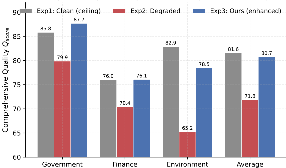
Quality Recovery from Degraded Data (Exp1 vs Exp2 vs Exp3)
