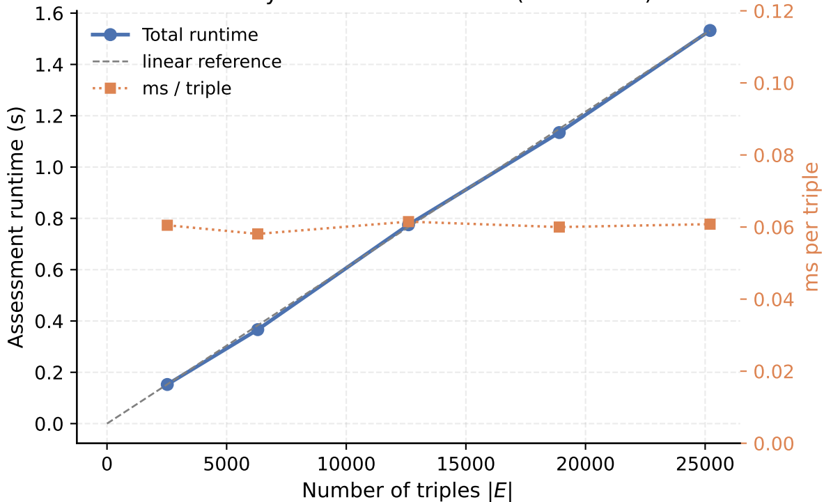
Scalability: Runtime vs KG Size (near-linear)
