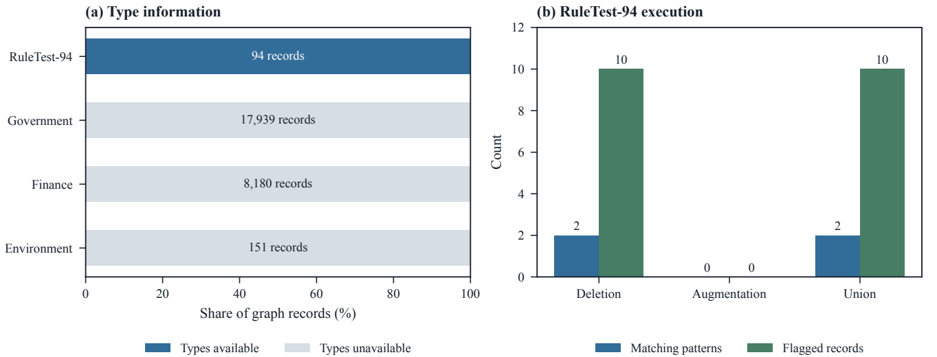
Fig. 6. Archive-rule integration audit. (a) Availability of endpoint types in each graph snapshot; numbers inside bars are record counts. (b) Exact matching patterns and flagged records on RuleTest-94. Missing type information causes abstention and is not scored as correct validation.
