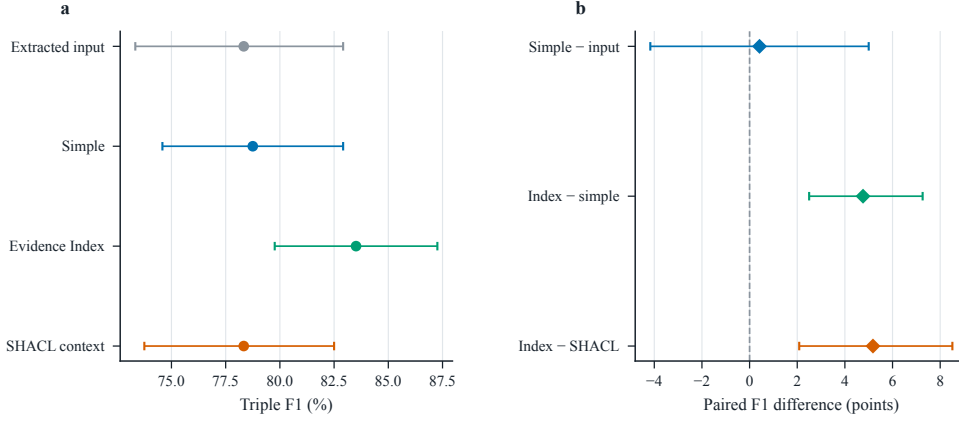
Fig. 9 Follow-up on new receipts. Left: mean triple F1 with 95% document-bootstrap intervals. Right: paired F1 changes; intervals resample whole documents. All repair methods share field definitions and source lines.
