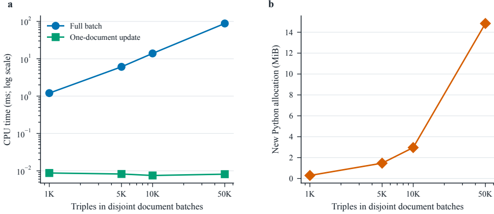
Fig. 7 Scaling of input-derived diagnostics on disjoint document batches. Local updates recompute one document. Memory records new batch allocations with shared source text.
