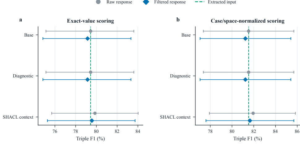
Fig. 8 Repair on independent receipt text. Points show mean triple F1 and 95% document-bootstrap intervals. Raw and gated results share model responses; the dashed line marks the extracted input.
