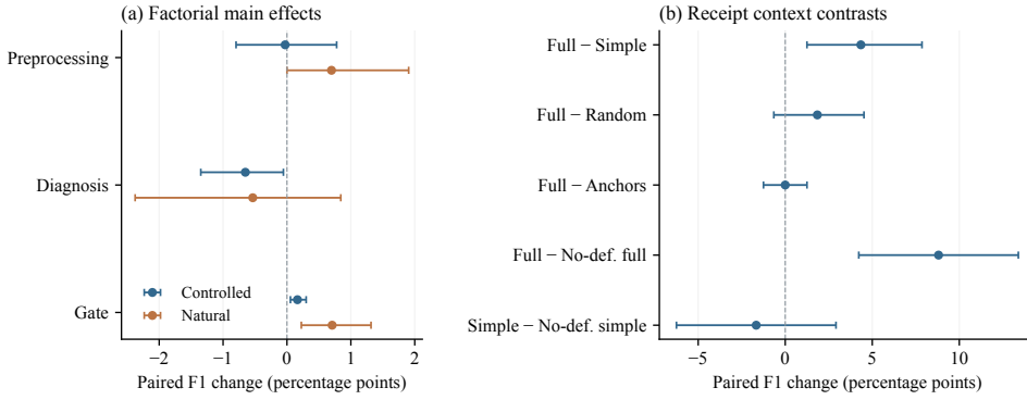
Fig. 10 Completed recovery controls. Points show paired mean F1 differences and bars show marginal 95% document-bootstrap intervals. Main-effect and receipt-contrast families receive separate Holm corrections; intervals are not multiplicity-adjusted.
