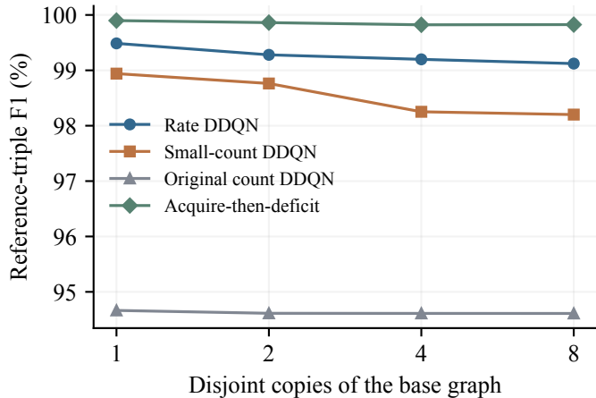
(a) Fixed-policy transfer
