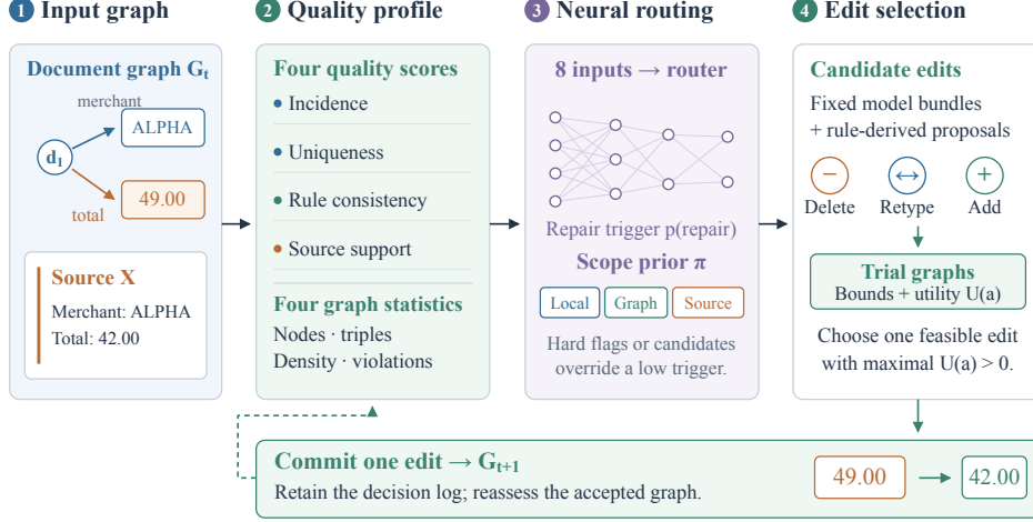
Fig. 1 Separately evaluated profile-based sequential repair. Four quality scores and four graph statistics feed a learned repair trigger and scope prior. Model edit bundles and rule proposals are evaluated on trial graphs; each round commits the feasible edit with the highest positive utility and reassesses the accepted graph. The field values and network drawing illustrate the mechanism. Section 4.4 describes its fixed-proposal evaluation.
