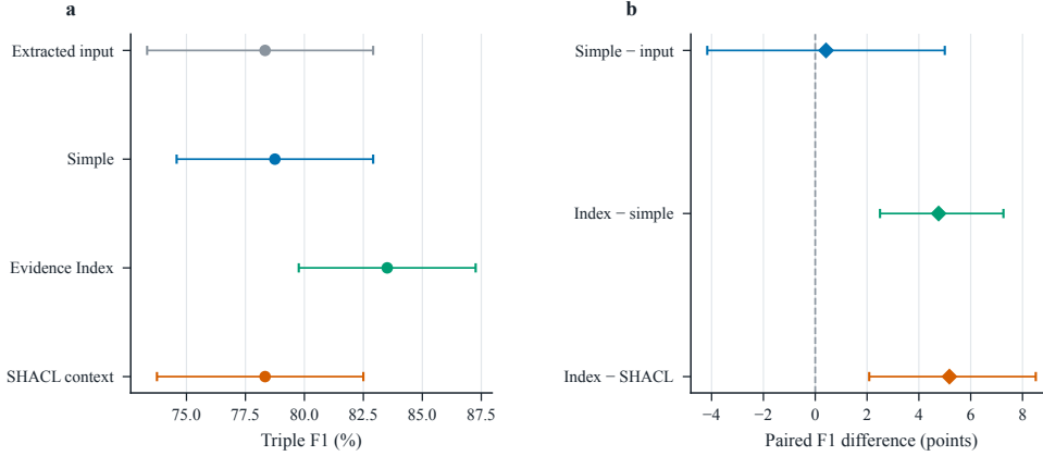
Fig. 8 Follow-up on new receipts. Left: mean triple F1 with 95% document-bootstrap intervals. Right: paired F1 changes; intervals resample whole documents. All repair methods share field definitions and source lines.
