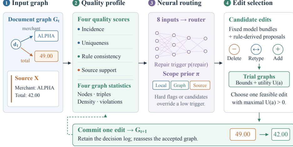
Fig. 1 Repair by choosing edits one at a time. Four quality scores and four graph counts feed the learned router. It gives a repair score and weights for three kinds of edits. The selector tries model and rule edits on graph copies. It applies the allowed edit with the highest positive score, then checks the graph again. Section 4.4 gives this test.
