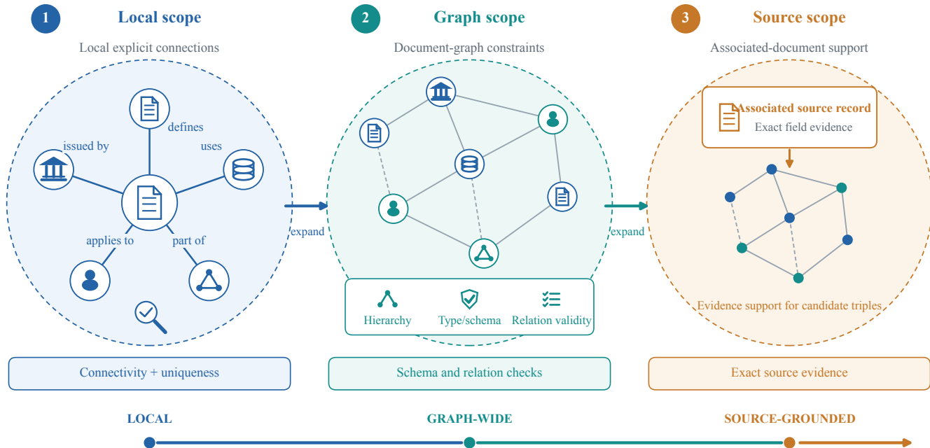
Three evidence scopes within one document-level knowledge graph.
