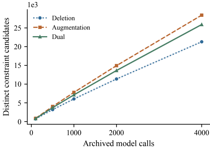
(a) Equal-call candidate diversity
