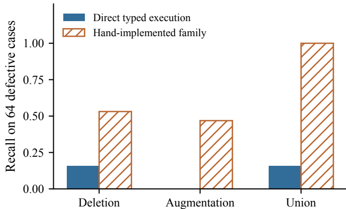
(b) Execution paths on RuleTest-94
