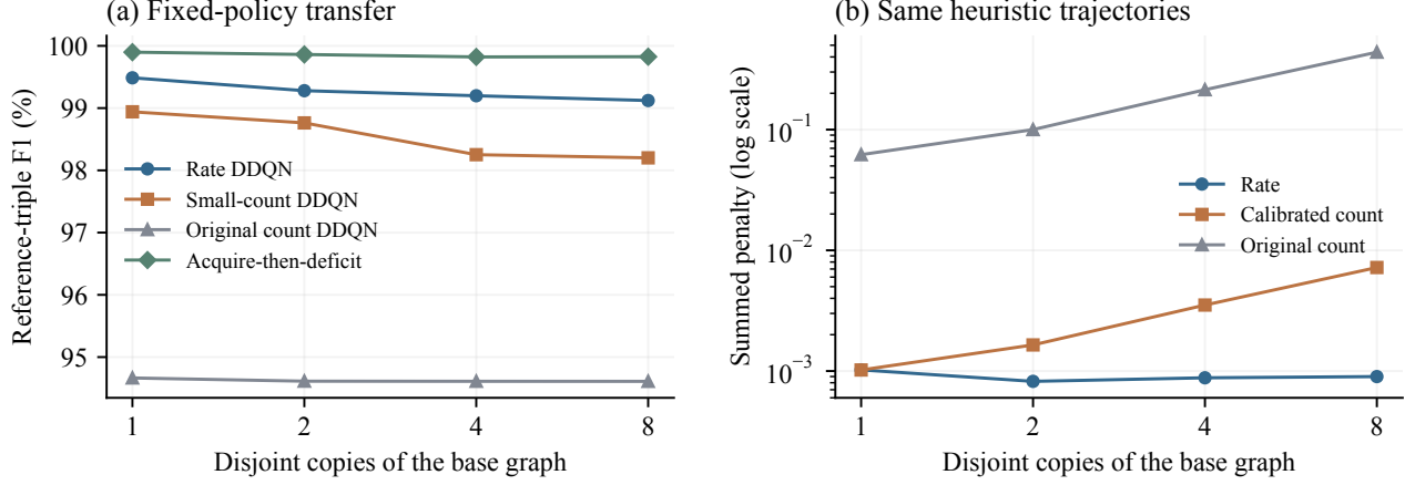
Fig. 6. Graph-size test with disjoint copies. (a) Mean F1 across ten model seeds and five scenarios per size. (b) Three penalties on the same heuristic action logs. All models train at the base size.
