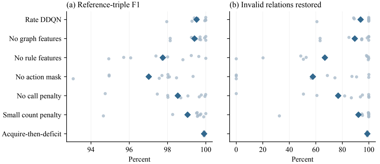
Fig. 5. Rate-reward component tests and small-count control. Dots show ten training-seed means; diamonds show their average. Each mean uses thirty shared scenarios. The heuristic uses a fixed rule.
