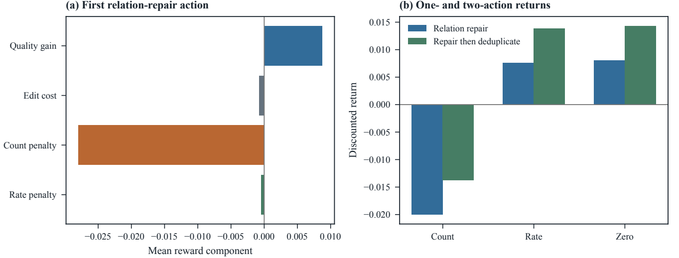
Fig. 3. Reward parts on ten earlier scenarios. Each trial starts from the corrupted input with four high-precision rules active. (a) Mean quality gain, edit cost, and each penalty for the first relation repair. (b) Return for that action and for repair followed by duplicate removal, with discount 0.95. Panel (a) shows the two penalties separately.
