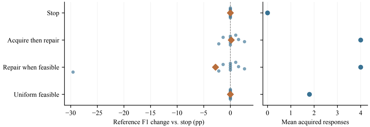
Fig. 9. Source-rule replay. Dots show ten episode F1 changes from stop; diamonds show their mean. The right panel counts acquired saved responses.
