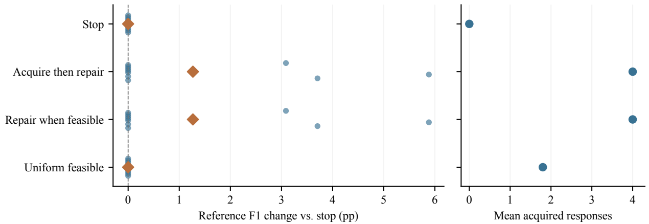
Fig. 10. Round 2 on the same ten development pairs. Both full schedules reach 95.69% mean F1 and keep every reference fact. Seven removals use type rules.
