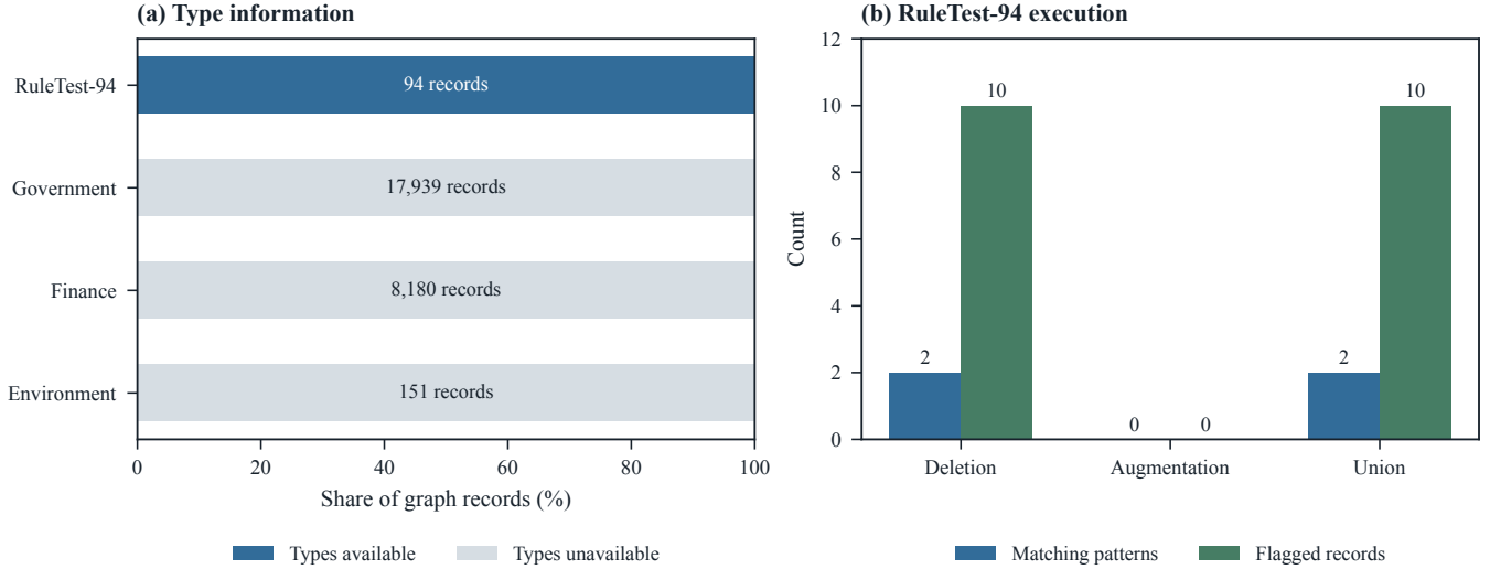
Fig. 8. Rule coverage. (a) Endpoint types in each snapshot; bar labels give record counts. (b) Matching patterns and flagged records in RuleTest-94. The checker skips records with missing types.
