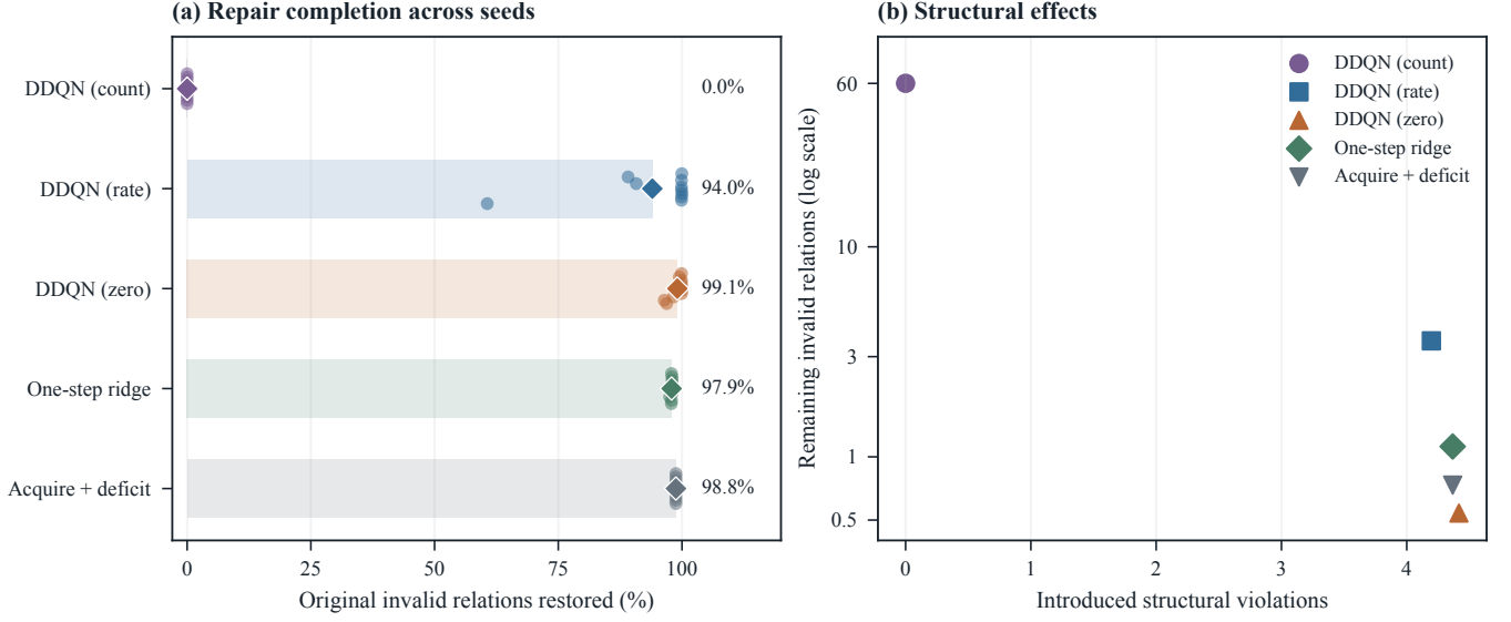
Fig. 4. Policy behavior on thirty new corruptions. (a) Original invalid edge copies restored and kept. Small dots show ten seed means; diamonds show their average. (b) New structural errors and remaining invalid relations. Each seed mean uses thirty scenarios. Panel (b) averages seeds and uses a log axis.
