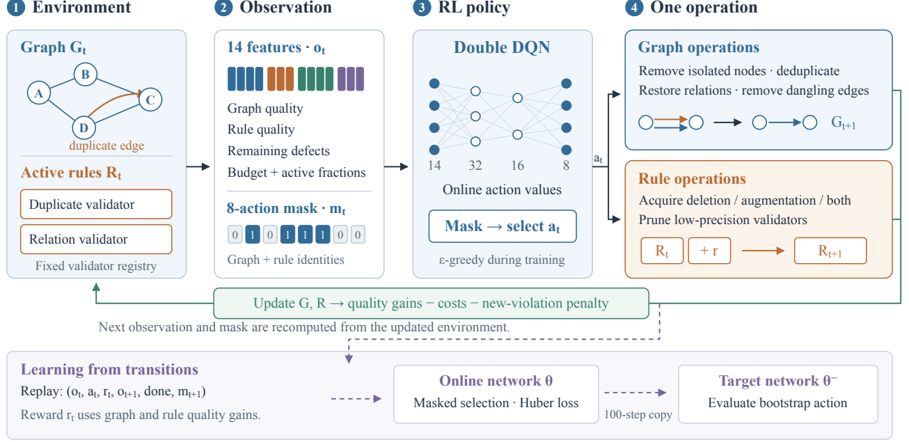
Fig. 1. Learning graph and rule actions. The environment gives fourteen inputs and a mask of eight actions. The policy chooses one action. The environment updates quality and reward. The lower band shows Double-DQN replay training. Small graphs and mask entries show example states. The loop uses a fixed rule library. Figure 2 gives the text prompts.
