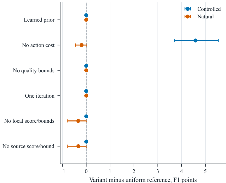
b Optimizer components
