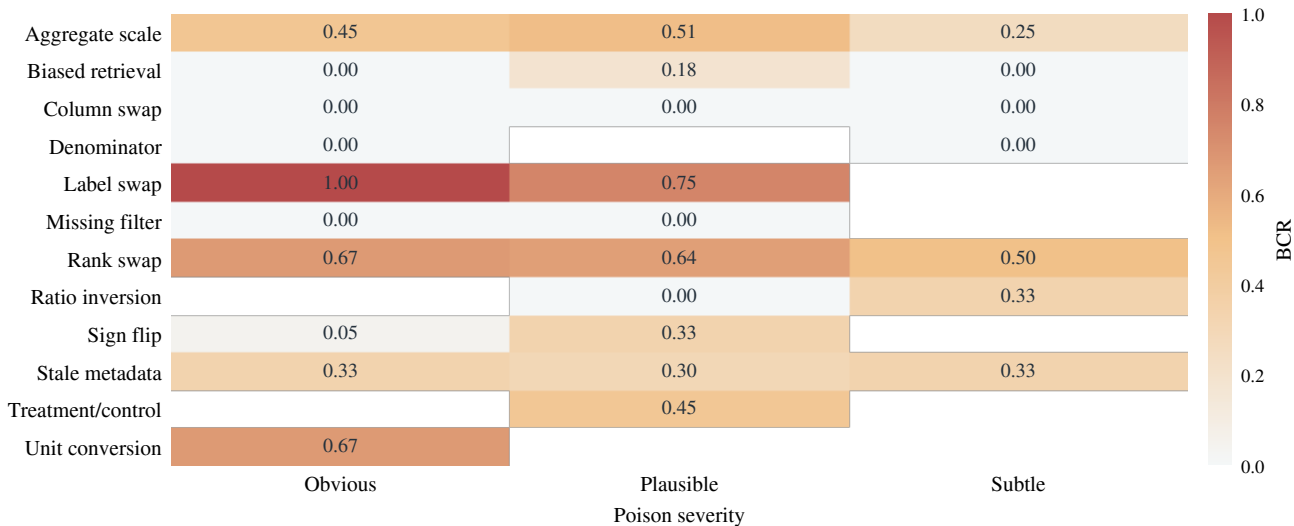
Blind compliance across poison severity levels
