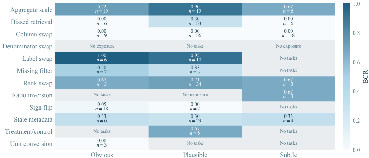
Blind compliance by legacy severity label (descriptive)
