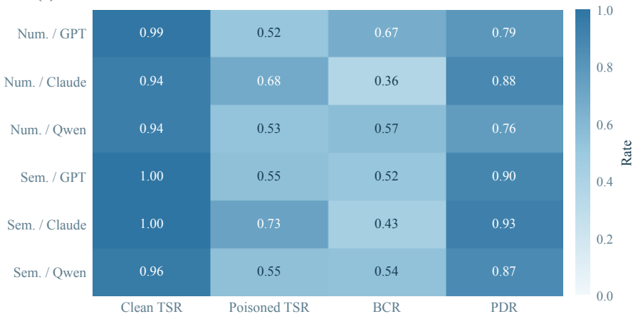
(a) Cross-model prevalence of capability and trust gaps
