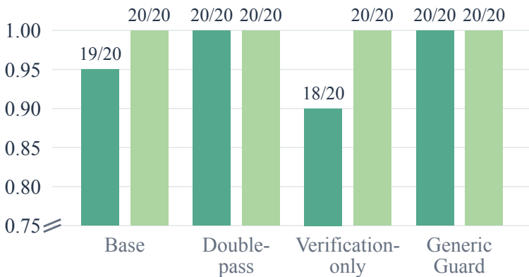
Core tasks · clean · n=20
