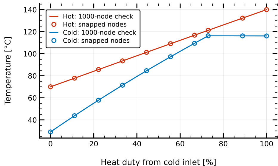
Partial evaporation / condenser
