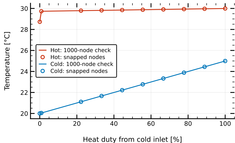
Partial evaporation / condenser
