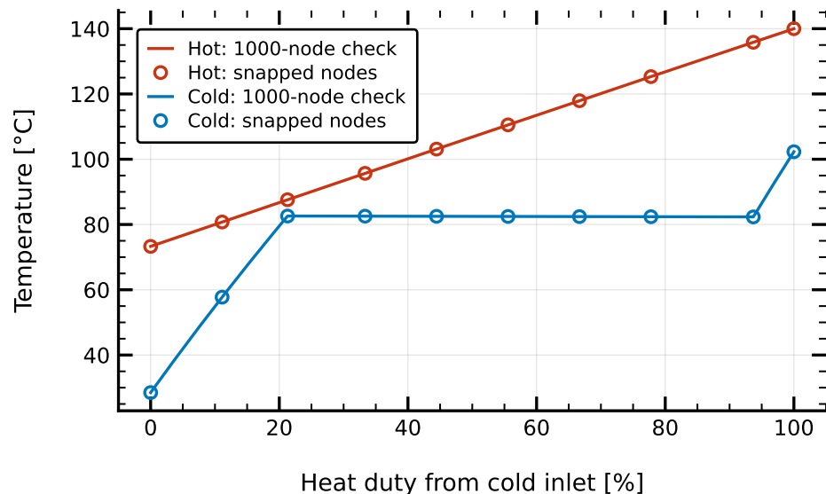
20 K superheat / condenser
