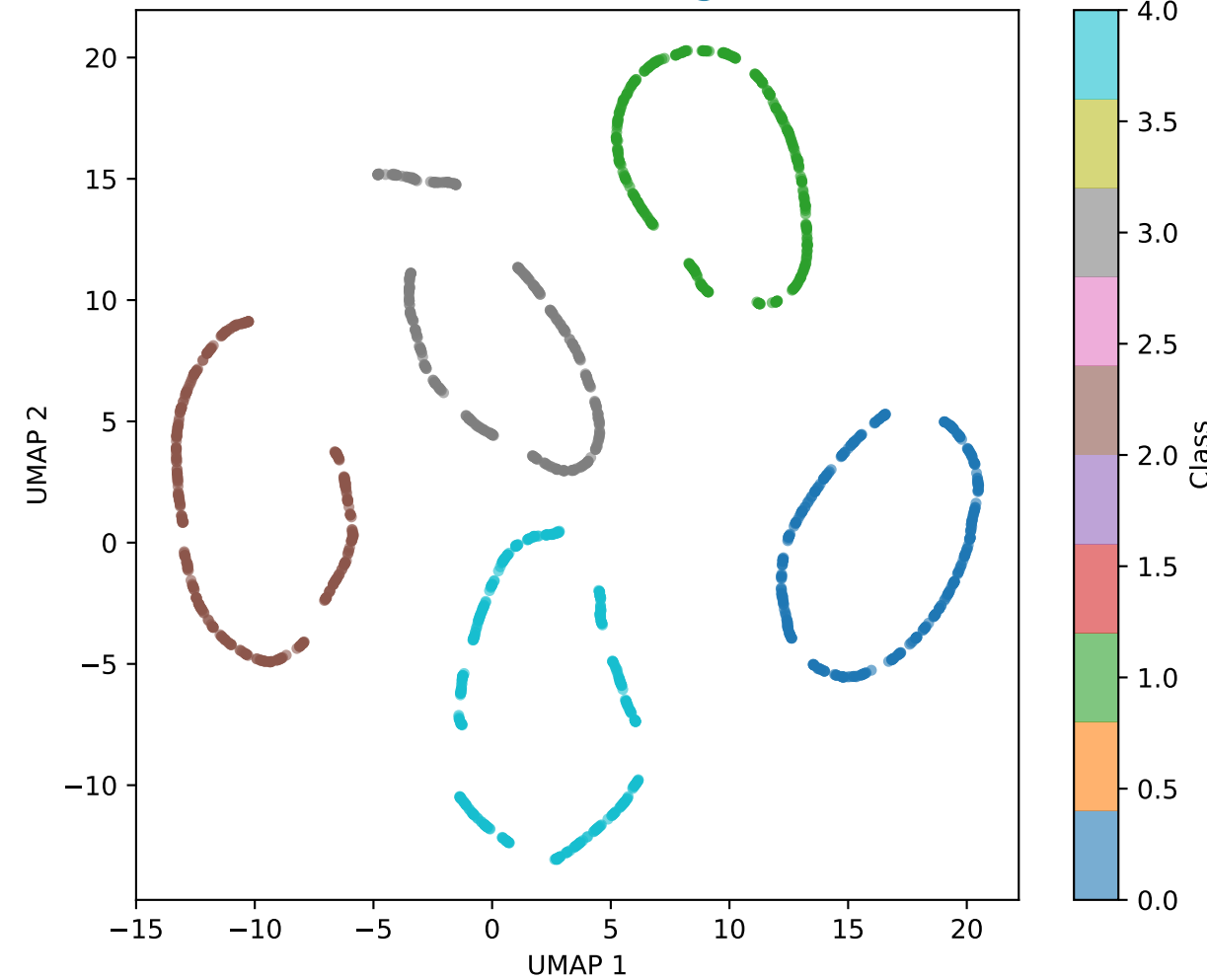
VAE Embedding
