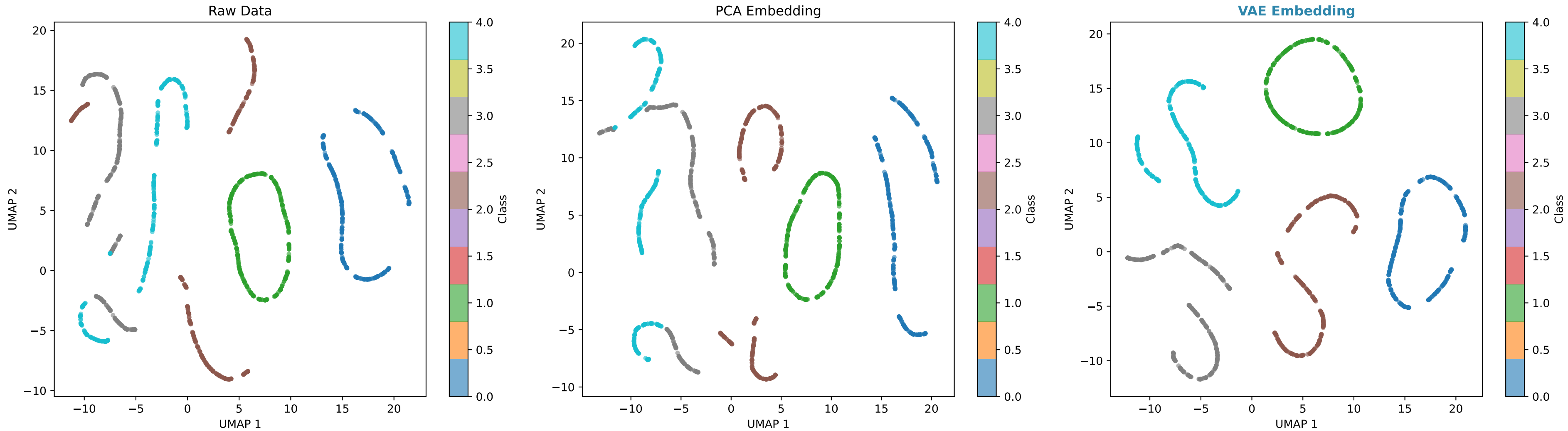
gmm_cnn_concentric_triangles_1 - ConcentricTriangles
