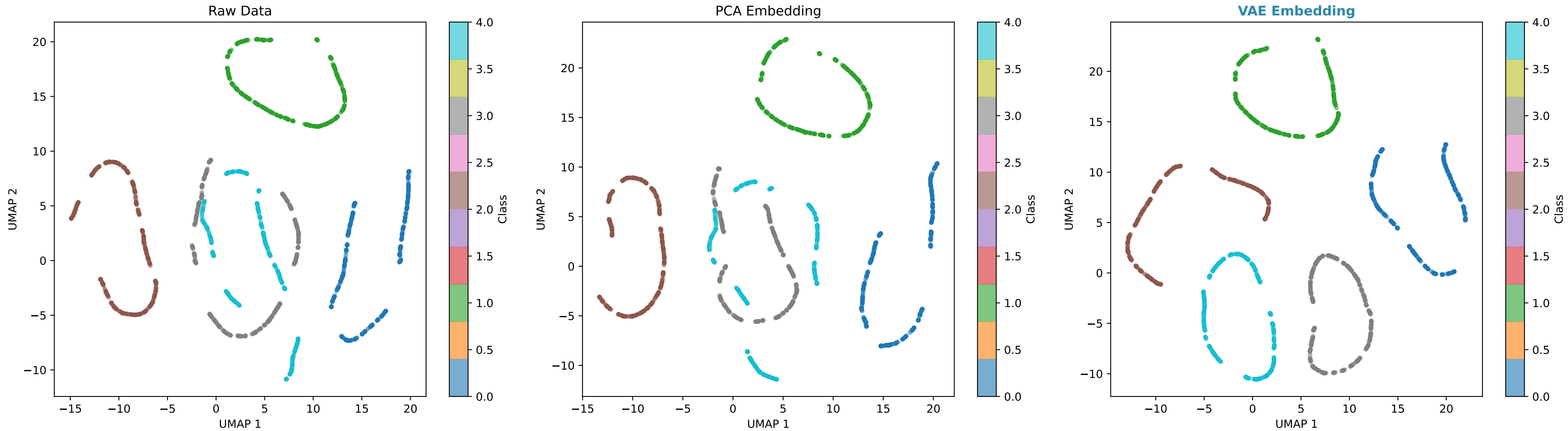
gmm_cnn_concentric_triangles_4 - ConcentricTriangles
