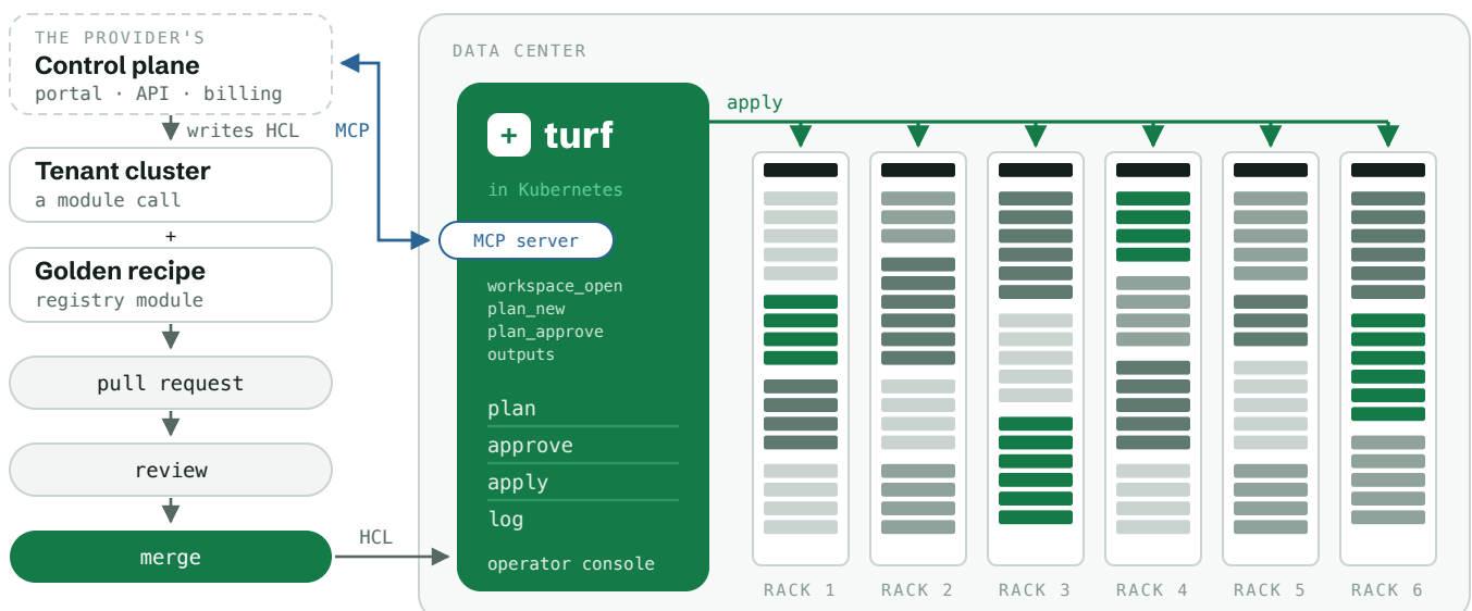
Figure 9. A tenant order, in the data center. The provider's control plane writes the tenant's cluster as HCL, merges it by pull request, and calls Turf's MCP server. Turf, beside the racks it runs, prepares the change plan and carries it out. Each block is a tenant cluster, and the green ones have a run in flight.
