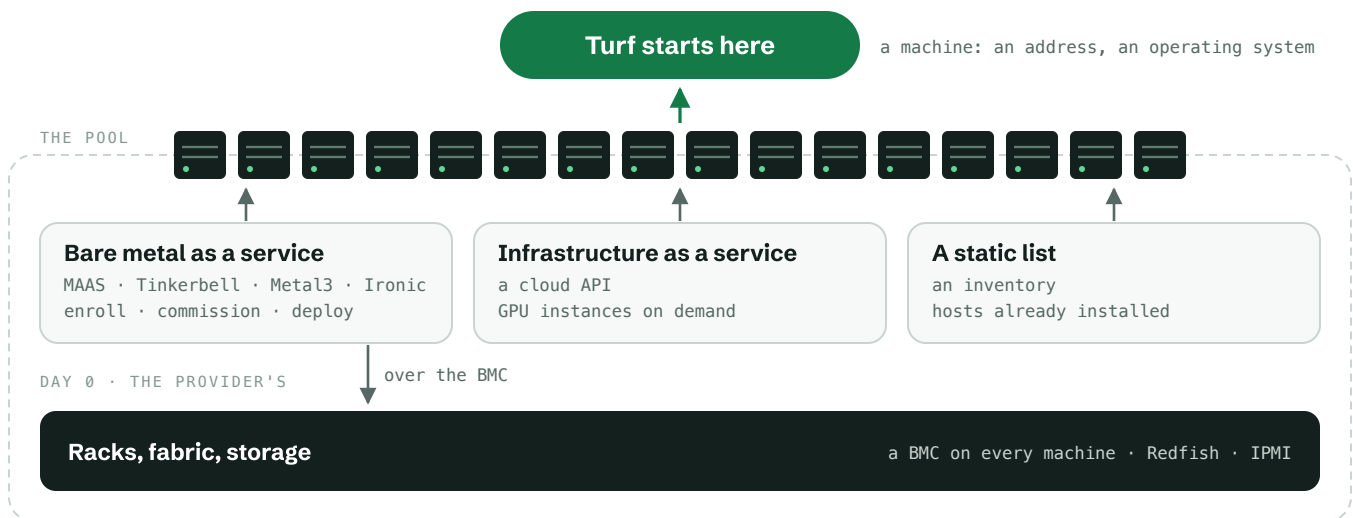
Figure 2. Pools of inventory. Day 0 is the provider's. Hardware reaches the stack as a pool of machines, offered by a bare-metal service, a cloud API or a static list. Turf starts where the pool hands over a machine.
