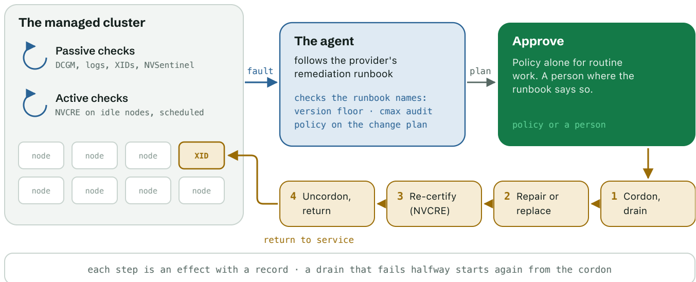
Figure 7. Two loops and one runbook. Detection belongs to the checks. The decision belongs to the provider's runbook. Turf carries it out, one approved, recorded step at a time.
