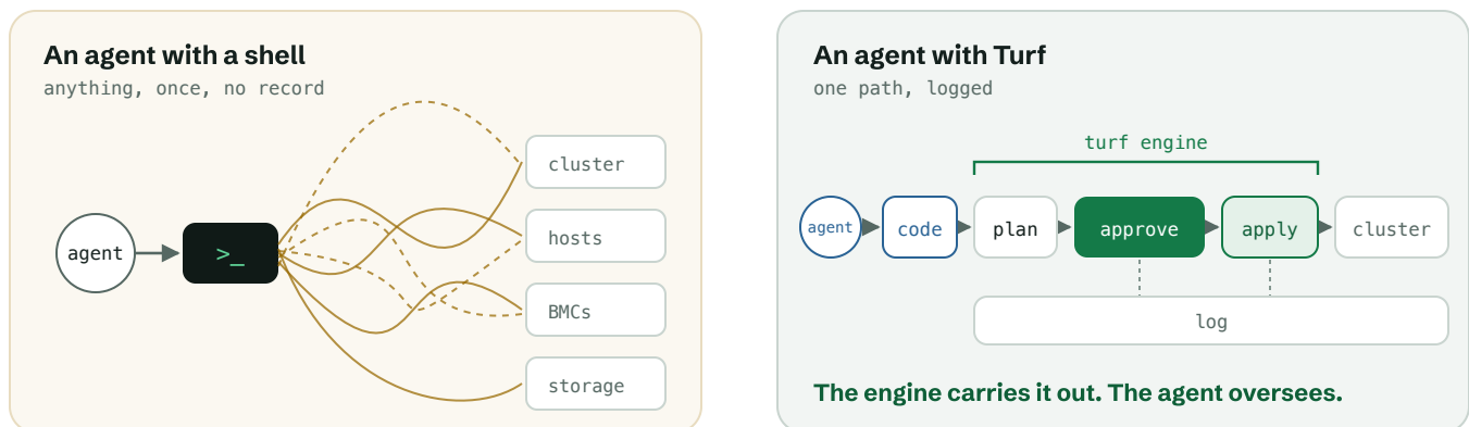
Figure 8. Vibecoded and governed. The same agent, acting through a shell, or editing the configuration so that the Turf engine prepares a change plan and carries it out.
