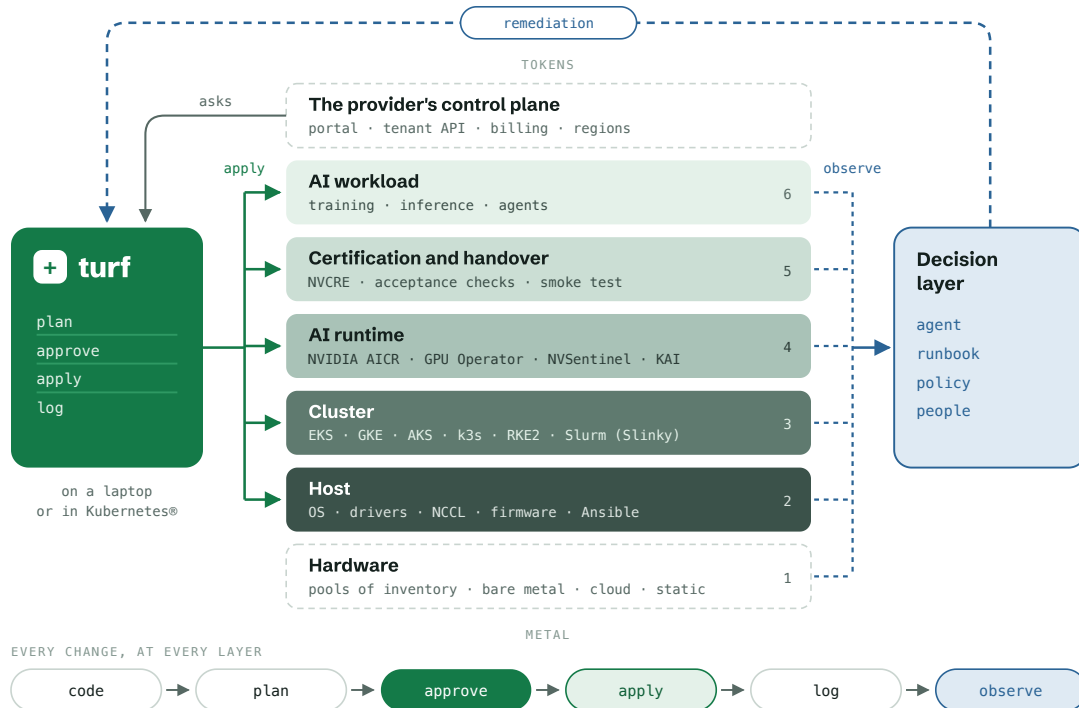
Figure 1. Metal to tokens. Every layer is code, brought up by one convergence loop. Turf runs on a laptop or in a Kubernetes® cluster. The decision layer (the provider's agent, runbook and policy) approves each change plan and oversees remediation. The dashed layers are the provider's own: hardware, offered as pools of inventory on day 0, and the control plane that asks Turf for clusters.
