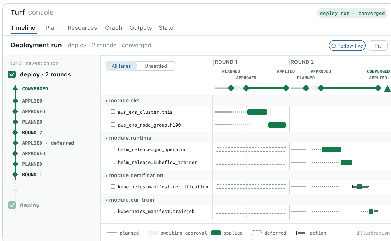
Figure 5. The convergence loop, in the Turf console. Round 1 builds the EKS cluster and defers everything that runs on it. Round 2 plans the deferred work, its change plan is approved, and the run converges.
