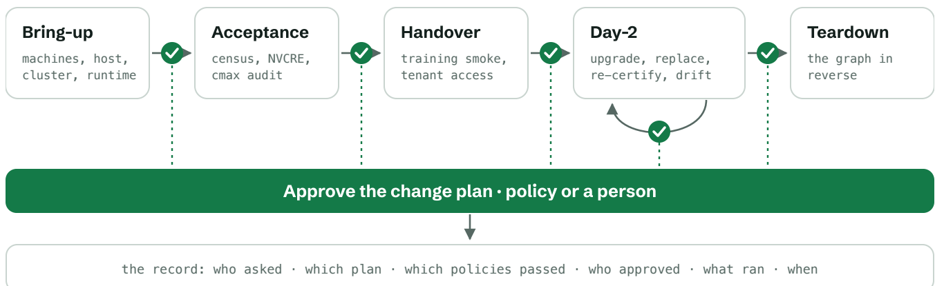
Figure 4. The managed-cluster lifecycle. Every transition is a change plan, approved and recorded.
