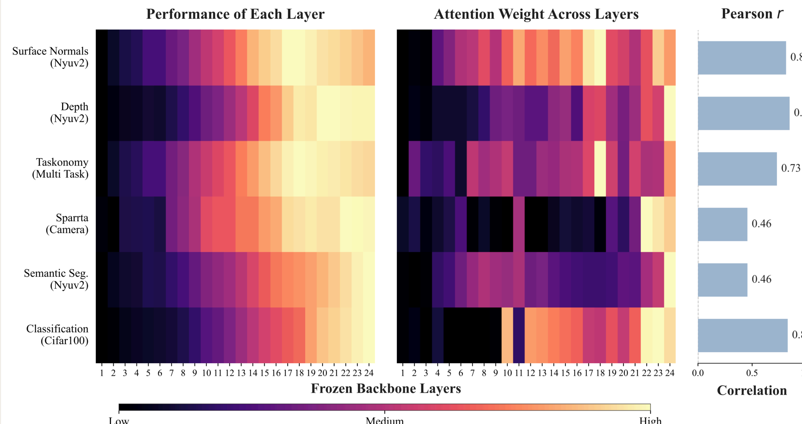
Fig. 5: Measured on an earlier AMDF variant (with per-layer refinement). AMDF's learned depth-attention (middle) tracks per-layer probe performance (left) on DINOv3-L/16. Alignment (Pearson r , right) is strongest for dense geometric tasks (depth r=0.85 , normals r=0.81 , Taskonomy r=0.73 ) and classification ( r=0.83 ), weaker for camera and segmentation ( r=0.46 ). Datasets differ from the tables (e.g. CIFAR-100, SpaRRTa).
