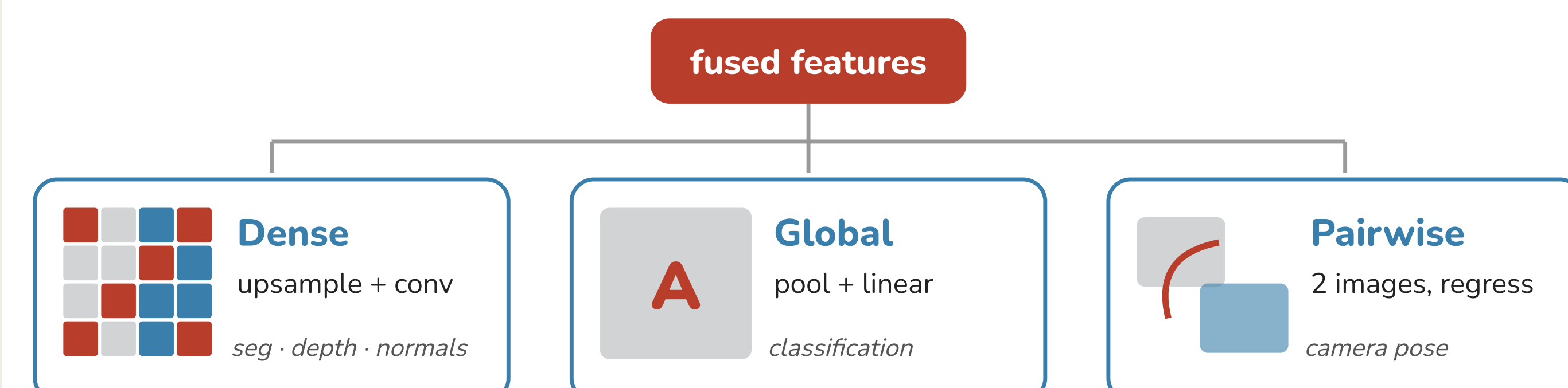
Fig. 4: The backbone stays frozen and all ViT blocks are used; only the fusion probe and the task head are trained.
