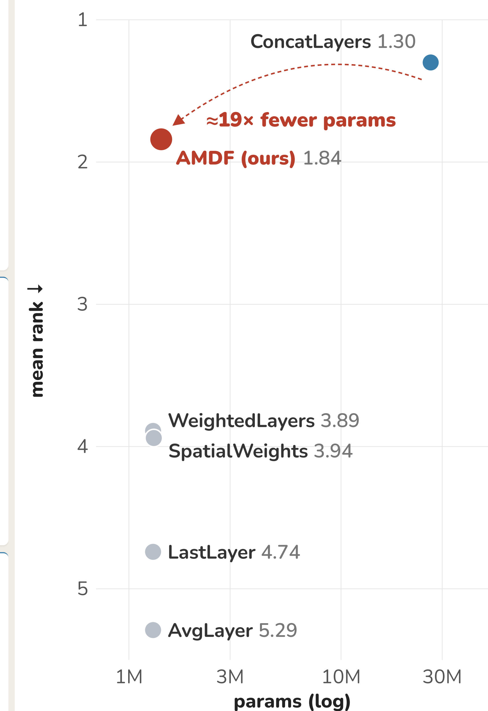
Fig. 7: ViT-L, all 5 tasks: ≈19x (pose head larger; ≈22x on dense tasks).
