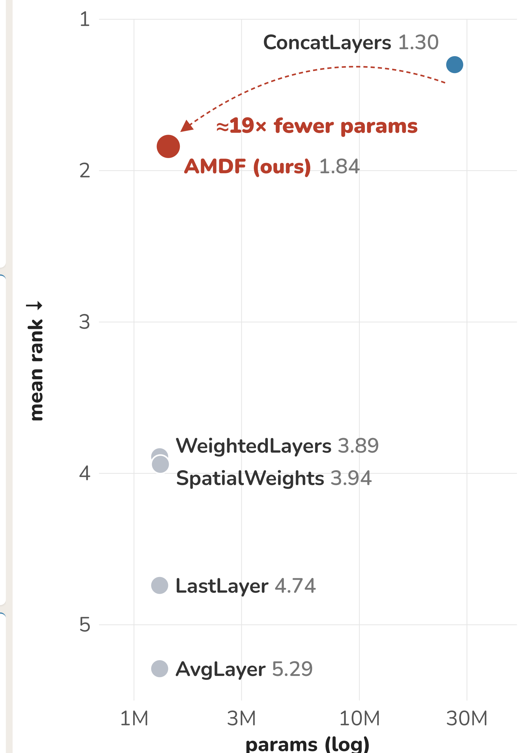
Fig. 7: ≈19× fewer params than Concat (5-task average, DINOv3-L).
