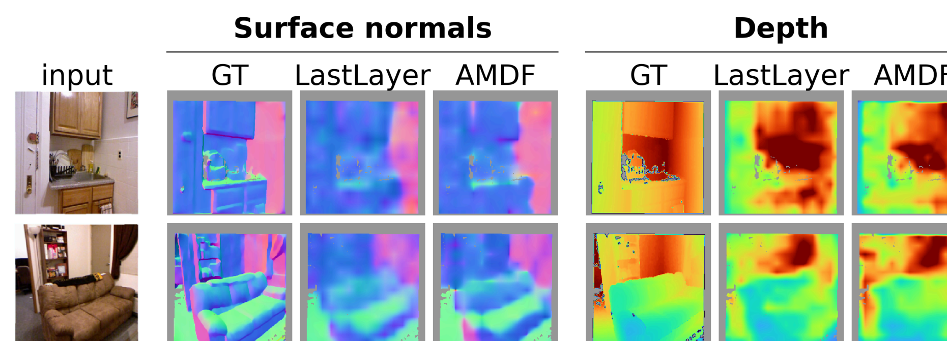
Fig. 5: NYUv2, DINOv3-L (seed-8 retrain, same config): AMDF's normals are sharper than LastLayer's; depth differs little.
